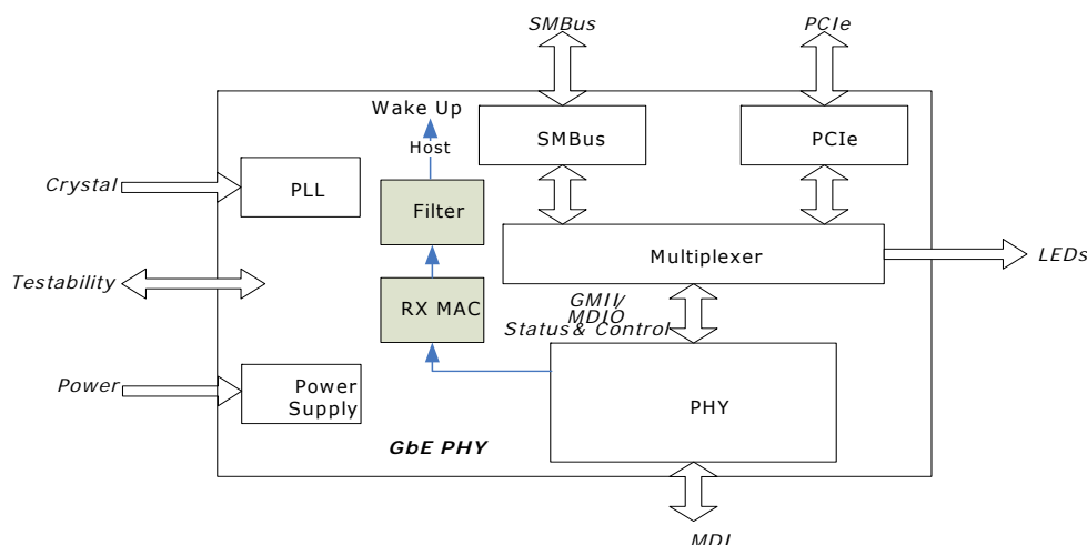
Figure 1. 82578 Block Diagram
